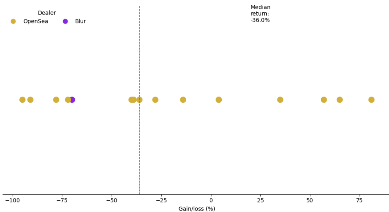
Distribution of loss and gain per repeat sale of The Currency in March
